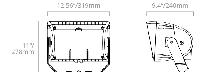
AFL 200W/240W with Optional Yoke
