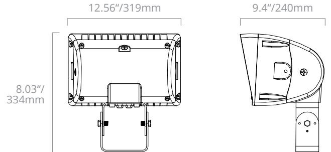
AFL 200W/240W with Optional Trunnion
