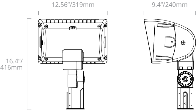
AFL 200W/240W with Optional Slipfitter for 2-3/8" pipe
